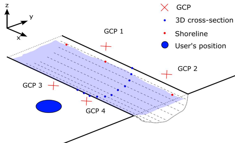
Data necessary for the setup of sites with irregular cross-section, namely the position of the Ground Control Points, points along the cross-section and optionally the position of three points along the shoreline on the far shore.
